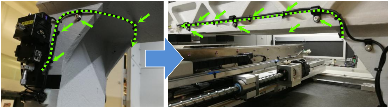
Figure 10 Sensor Amplifier Cable Routing
