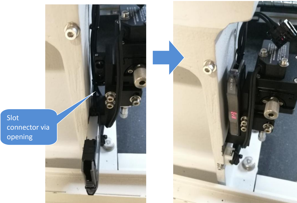
Figure 9 Sensor Amplifier Assembly
