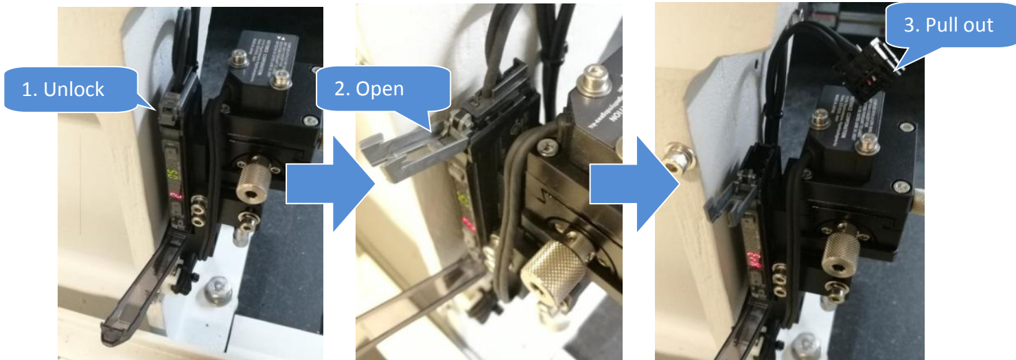
Figure 3 Sensor Head End Connector Removal
