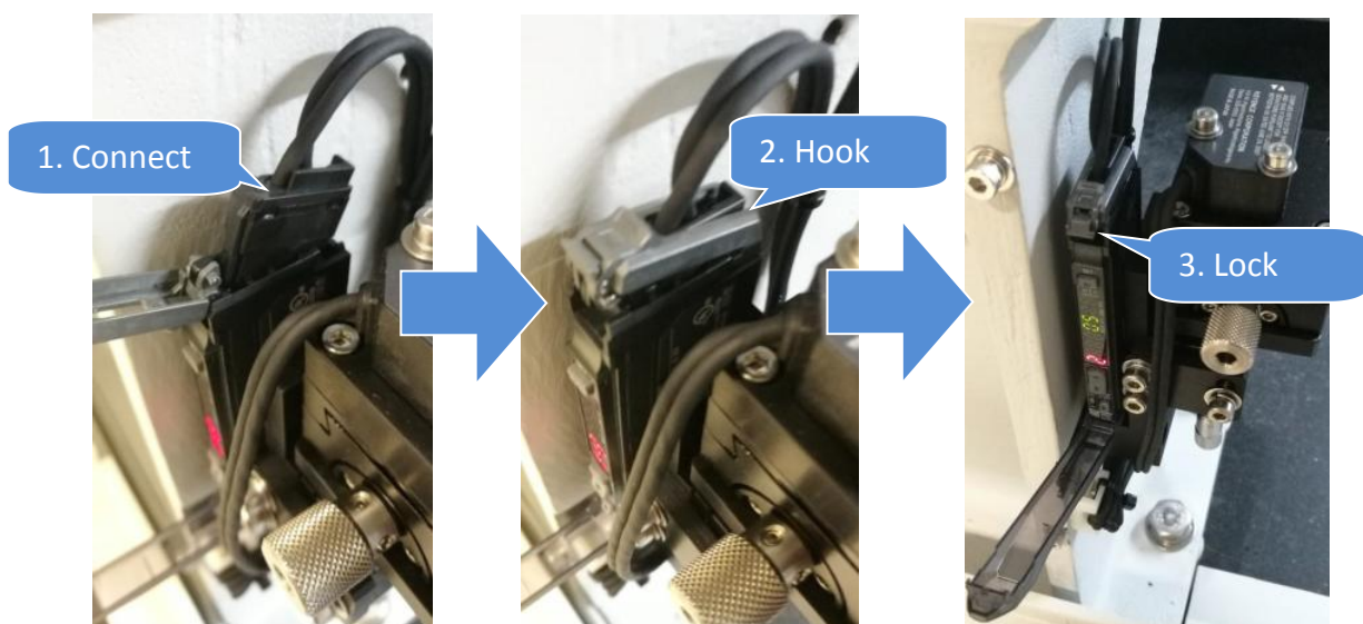
Figure 12 Sensor Head Connector Connect
