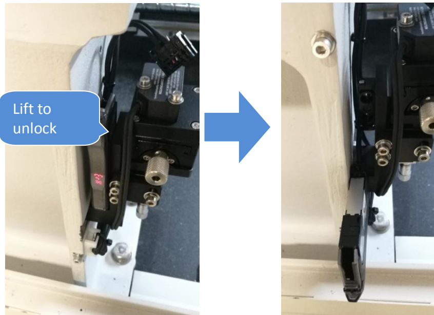
Figure 5 Sensor Amplifier Removal
